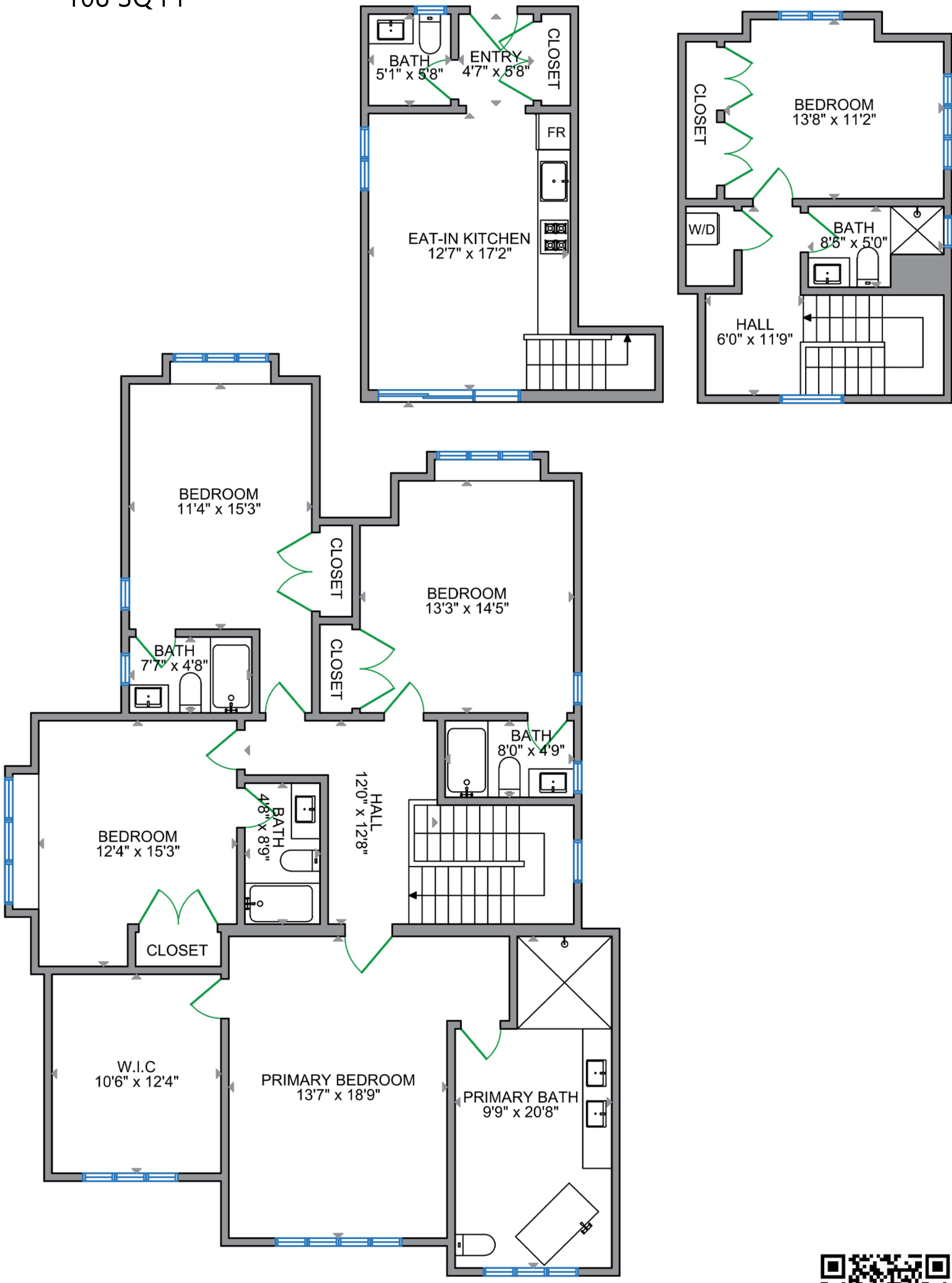
Upper Floor - 1668 SQ FT Ceiling height - 8'0" ~ 11'0"
